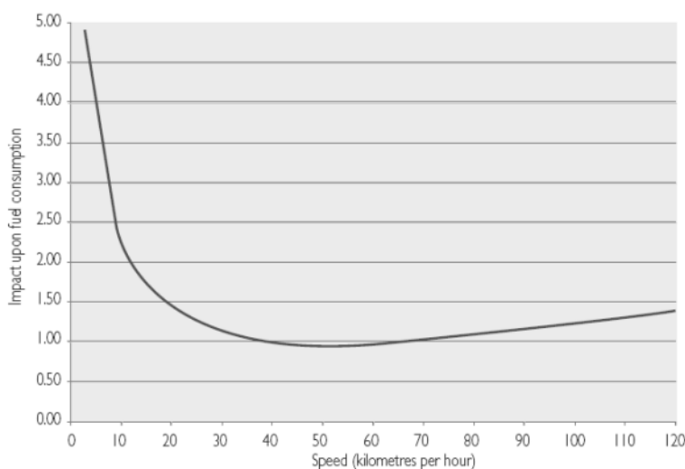
Figure 4: Fuel efficiency related to speed
