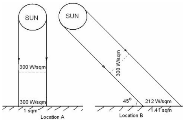
Figure 1: An illustration of the reduction of radiation intensity per square metre due to sun angle
