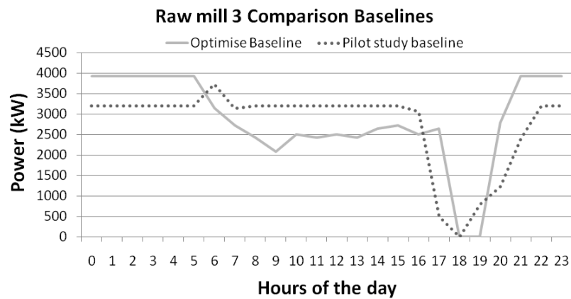
Figure 11: Comparative profiles
