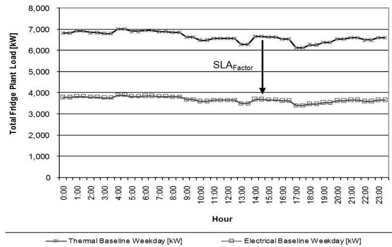
Figure 11: Thermal and electrical weekday baseline profiles
