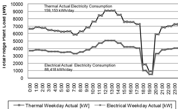
Figure 9: Thermal and electrical actual weekday profiles
