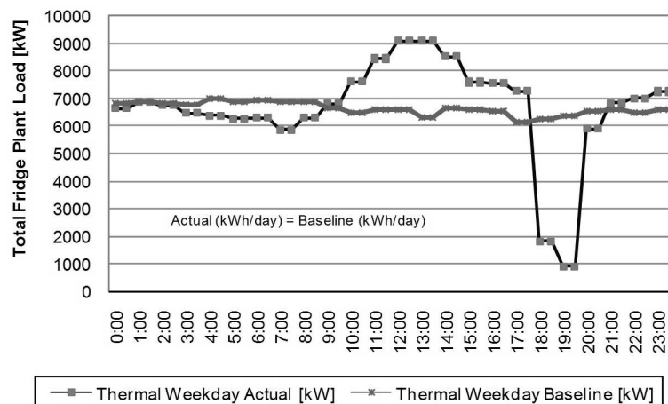
Figure 10: Actual and baseline profiles for the total fridge
